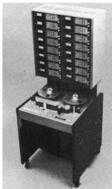
16-Kanal-Studiomaschine Studer A 80.
